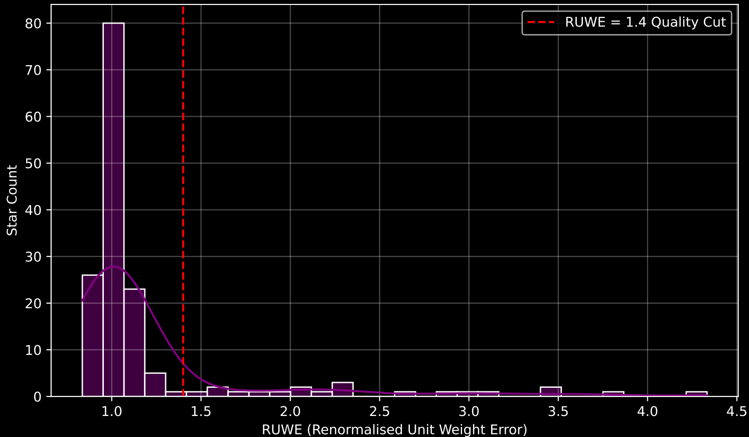
GALAH DR4 Field [528] RUWE Distribution (n= 155)
