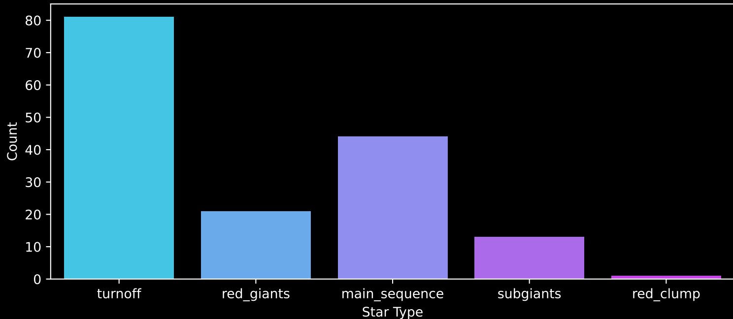
GALAH DR4 Field: [528] Count plot of Star Type
